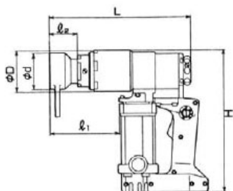
寸法図A
